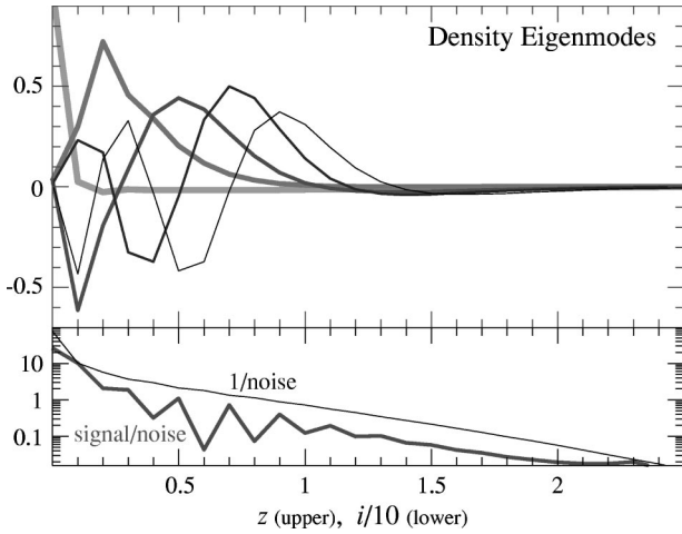
FIG. 3. Principle components of the dark energy density d \equiv \ln(\rho_{DE}/\rho_{crit}) : (upper) first five eigenfunctions of the growth function (thick to thin) plotted in redshift; (lower) rank ordered inverse rms noise \lambda_i^{-1/2} (thin) and signal-to-noise ratio.
